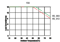
fig. 3. Thermal derating curve 15 A
