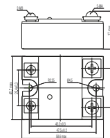
fig. 5. Dimension (mm)
