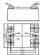
fig. 5. Dimension (mm)
