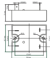
fig. 5. Dimension (mm)
