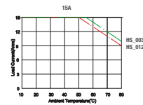
fig. 3. Thermal derating curve 15 A
