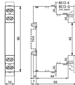
fig. 3. Dimension (mm)
