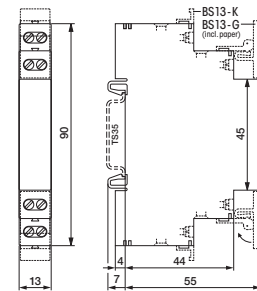
fig. 3. Dimension (mm)
