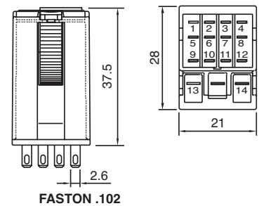
fig. 4. Dimension (mm)
