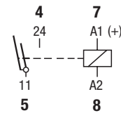
fig. 2. AC-1 voltage endurance
