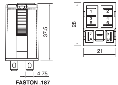
fig. 4. Dimension (mm)
