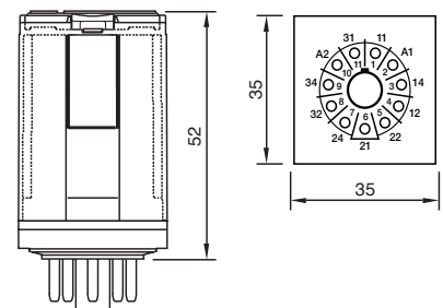
fig. 4. Dimension (mm)
