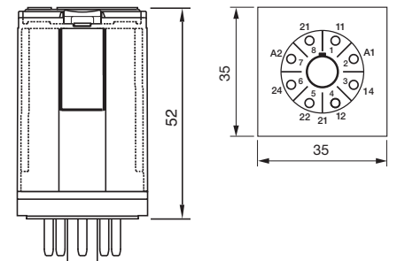
fig. 4. Dimension (mm)
