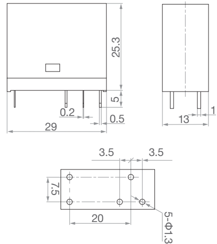
fig. 3. Dimension (mm)
