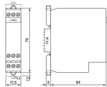
fig. 3. Dimension (mm)
