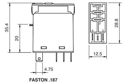
fig. 4. Dimension (mm)
