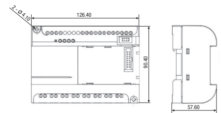
fig. 2. Dimension (mm)
