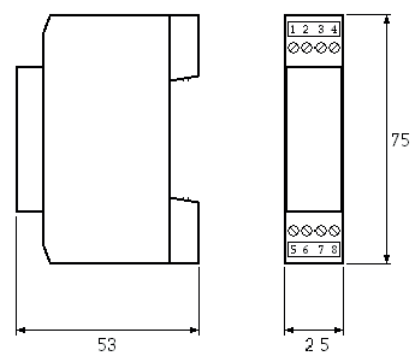
fig. 2. Dimension (mm)
