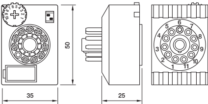
fig. 2. Dimensions (mm)
