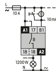
fig. 2. AC voltage endurance
