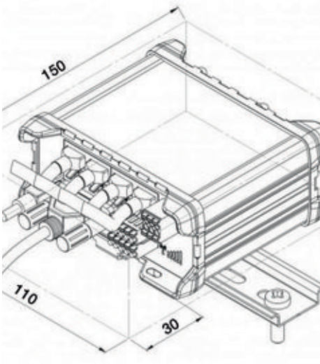
fig. 2. Dimensions (mm)
