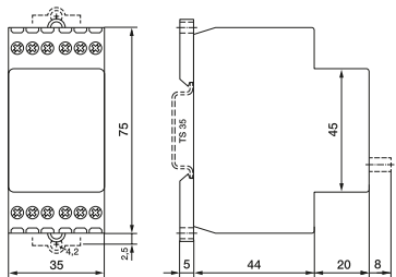
fig. 2. Dimensions (mm)
